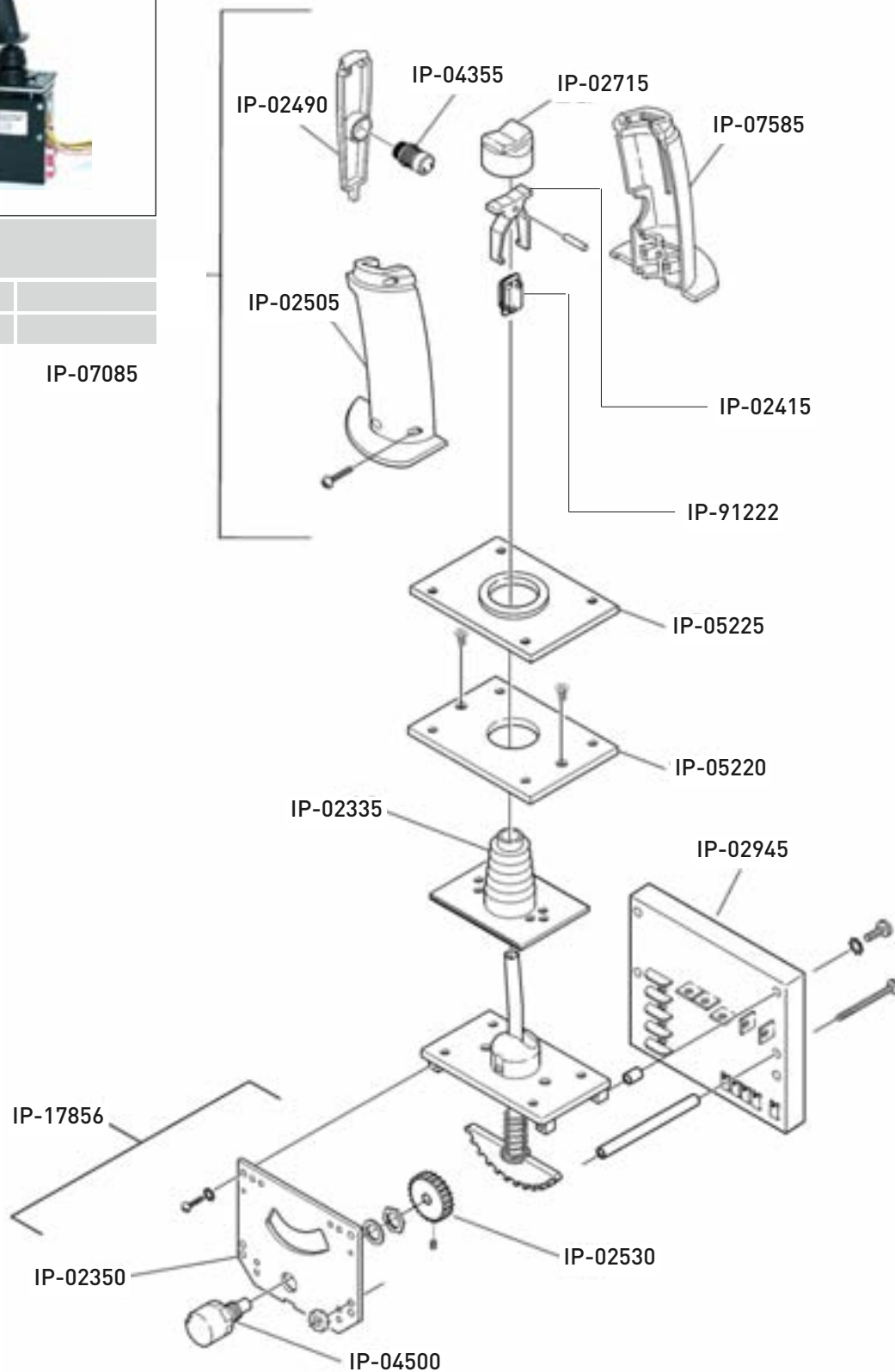
Controller
