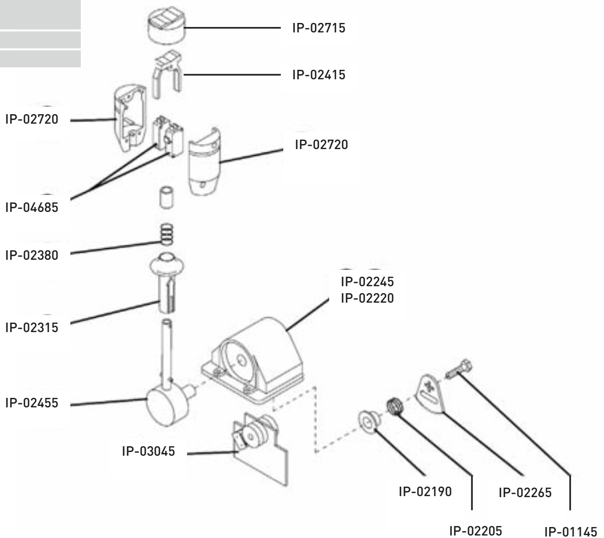
Controller
